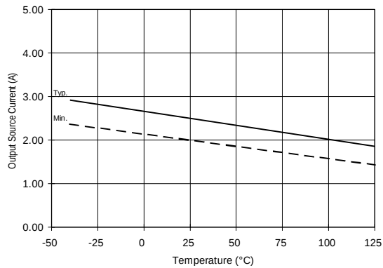
Figure 26A. Output Source Current vs. Temperature www.irf.com
