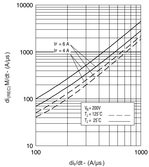
Fig. 7 - Typical di_{(REC)} M/dt vs. di_t/dt
