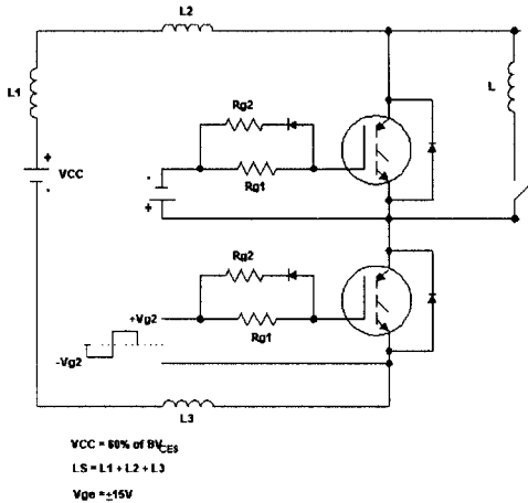
Fig. 17a - Test Circuit for Measurement of I_{LM} , E_{on} , E_{off(diode)} , t_{rr} , Q_{rr} , I_{rr} , t_d(on) , t_r , t_d(off) , t_f
