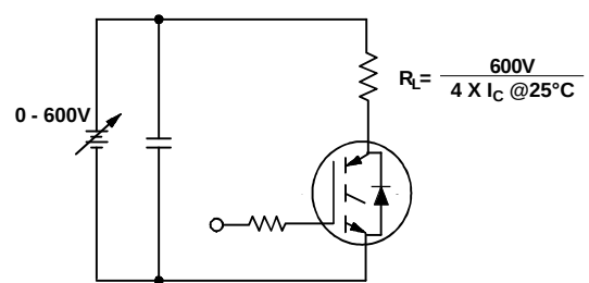
Figure 23. Pulsed Collector Current Test Circuit
