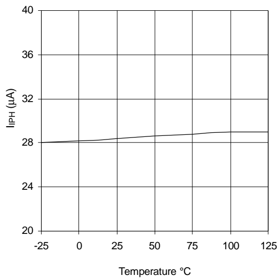
Graph 13. I PPH vs Temperature (IR2159/IR21591)
