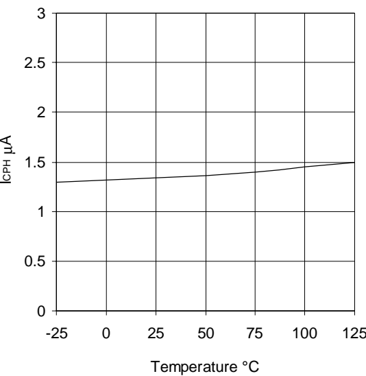
Graph 11. I_{CPH} vs Temperature (IR2159/IR21591)
