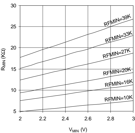
Graph 10. R_{MIN} vs V_{MIN}
