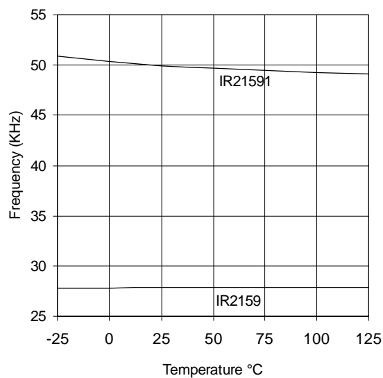
Graph 15. Frequency vs Temperature V VCO =0V (IR2159/IR21591)
