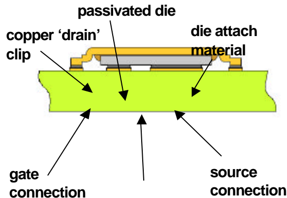
Figure 3.0 – Cross-section of DirectFET Soldered to PCB
