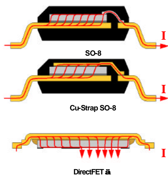
Figure 5.0 – Comparison of Current Conduction Paths for SO-8, Cu-strap SO-8 & DirectFET
