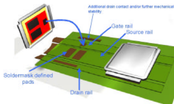
Figure 8.0 – Paralleling DirectFETs
