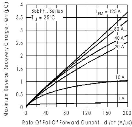
Fig. 10 - Recovery Charge Characteristics, T_J = 25^\circ C
