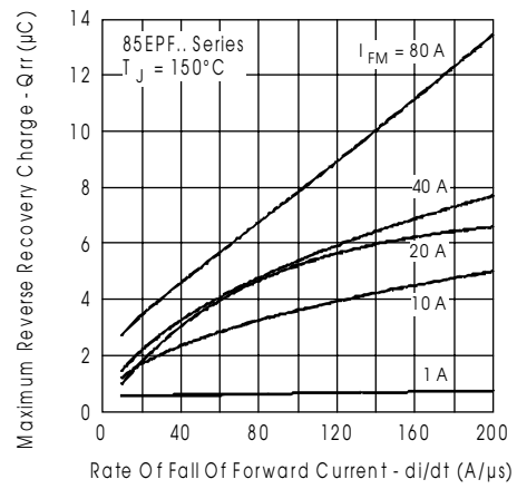
Fig. 11 - Recovery Charge Characteristics, T_J = 150^\circ C
