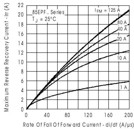
Fig. 12 - Recovery Current Characteristics, T_J = 25^\circ C
