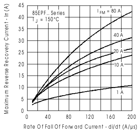
Fig. 13 - Recovery Current Characteristics, T_J = 150^\circ C
