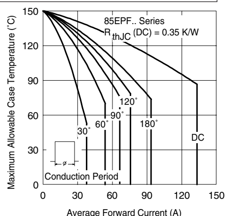
Fig.2-Current Rating Characteristics
