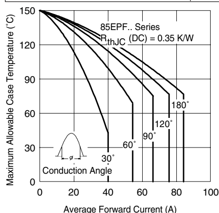
Fig.1-Current Rating Characteristics
