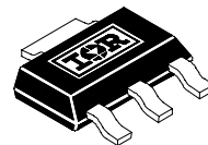
3 Lead SOT223
