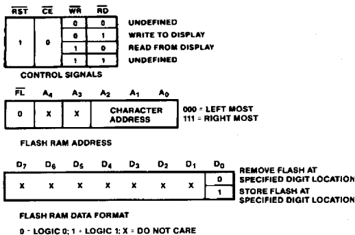
Figure 5. Logic Levels to Access the Flash RAM.
