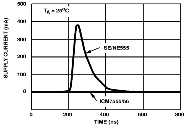
FIGURE 1. SUPPLY CURRENT TRANSIENT COMPARED WITH A STANDARD BIPOLAR 555 DURING AN OUTPUT TRANSITION
