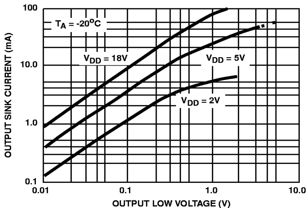
FIGURE 7. OUTPUT SINK CURRENT vs OUTPUT VOLTAGE
