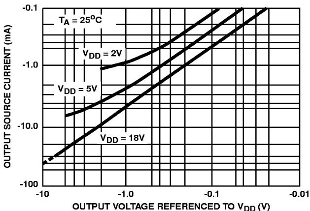
FIGURE 6. OUTPUT SOURCE CURRENT vs OUTPUT VOLTAGE
