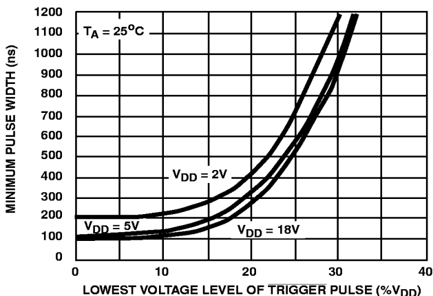
FIGURE 4. MINIMUM PULSE WIDTH REQUIRED FOR TRIGGERING
