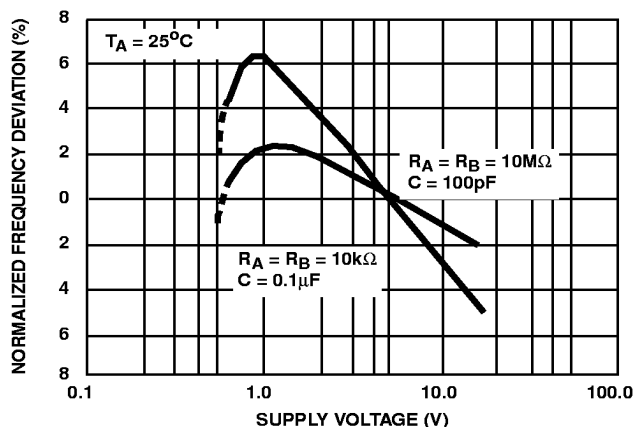
FIGURE 10. NORMALIZED FREQUENCY STABILITY IN THE ASTABLE MODE vs SUPPLY VOLTAGE
