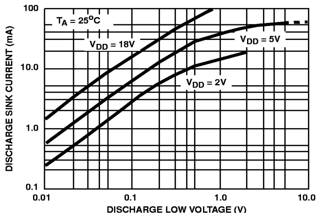
FIGURE 11. DISCHARGE OUTPUT CURRENT vs DISCHARGE OUTPUT VOLTAGE
