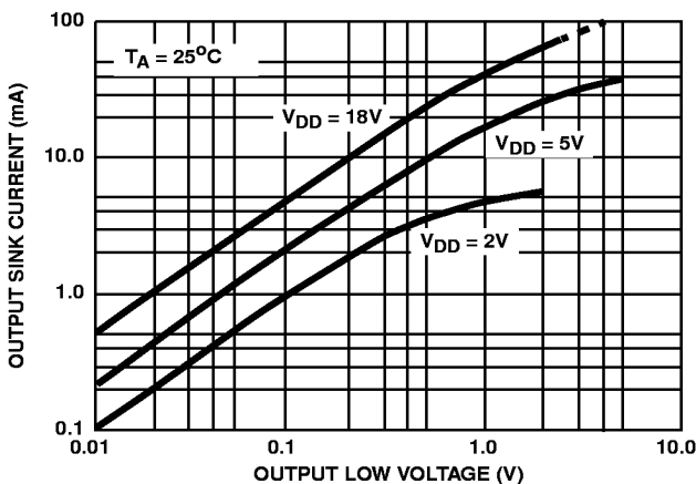
FIGURE 8. OUTPUT SINK CURRENT vs OUTPUT VOLTAGE
