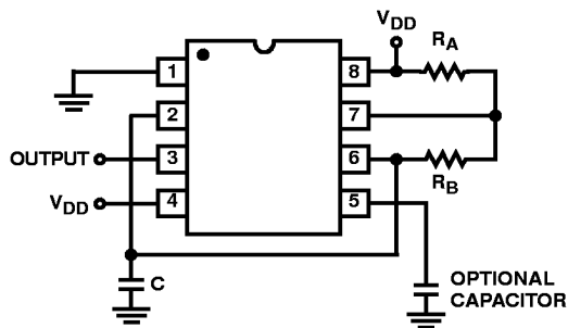
FIGURE 2B. ALTERNATE ASTABLE CONFIGURATION
