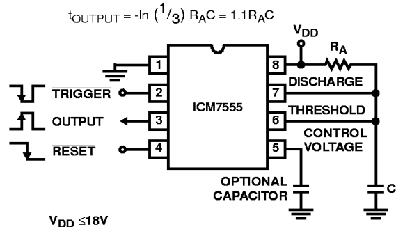
FIGURE 3. MONOSTABLE OPERATION
