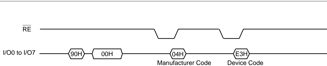
Figure 7 Read ID Operation
