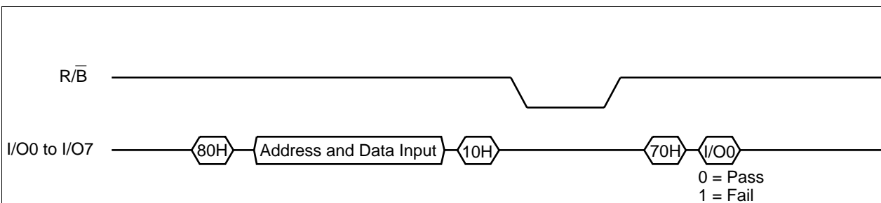
Figure 5 Page Program
