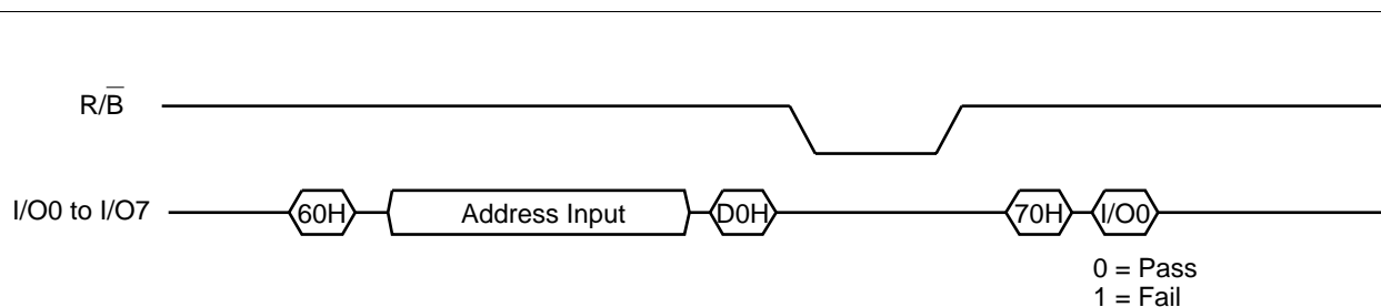
Figure 6 Block Erase
