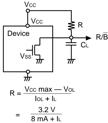
Figure 28 Termination for R/\overline{B}
