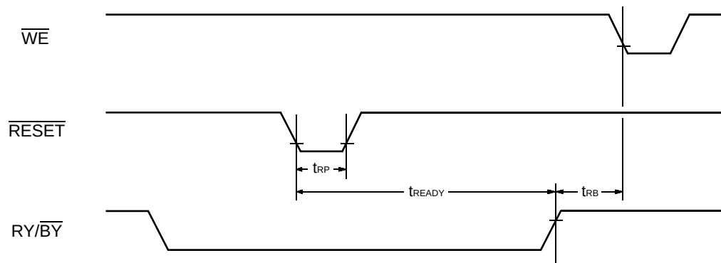
Figure 12 \overline{RESET} , RY/\overline{BY} Timing Diagram
