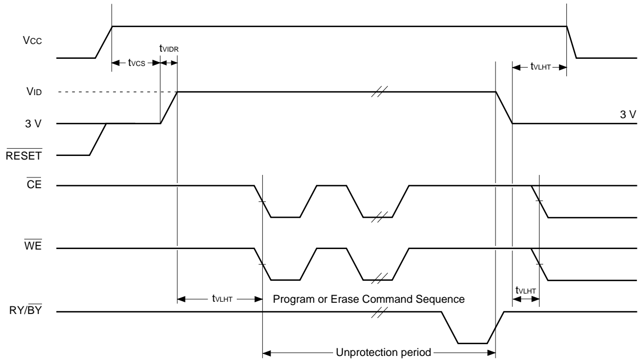
Figure 1 Temporary Sector Unprotection Timing Diagram
