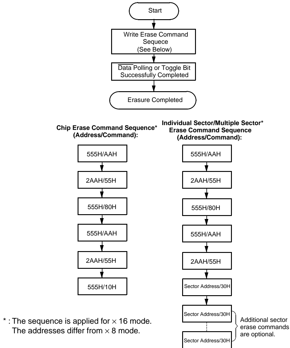
Figure 3 Embedded Erase™ Algorithm
