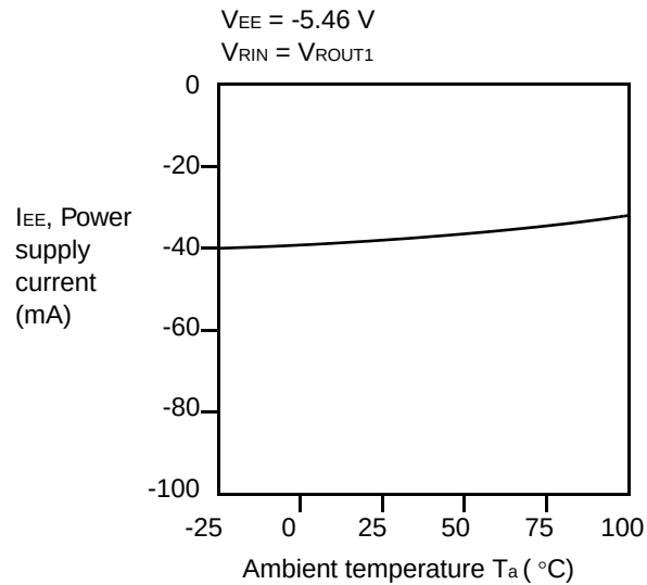
1. Power Supply Current v.s. Ambient Temperature
