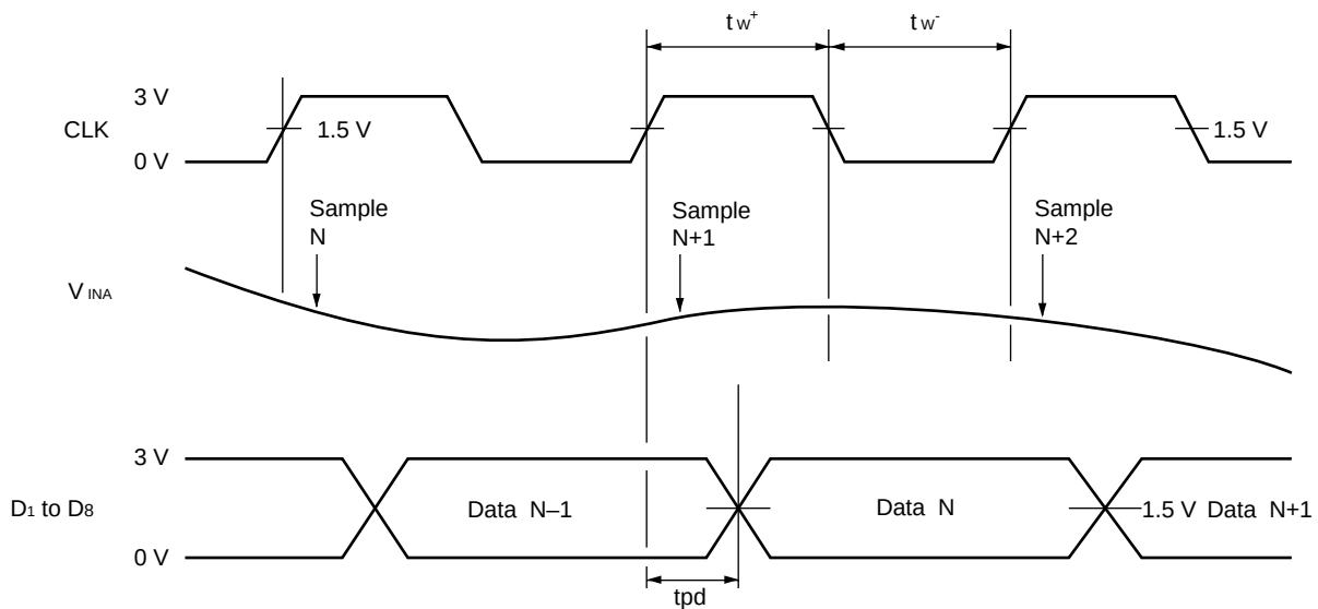
Figure 1 Timing Diagram
