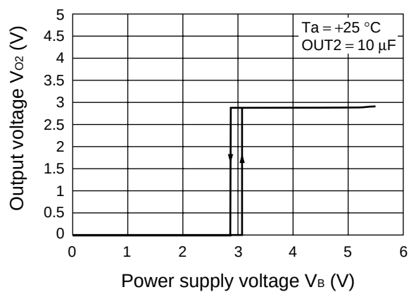
Output voltage vs. power supply voltage (BBREG2)
