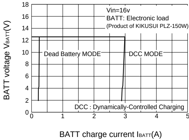
BATT voltage vs. BATT charge current
