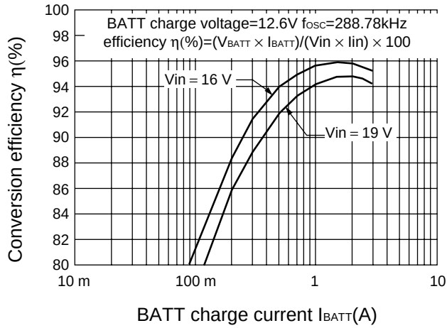
Conversion efficiency vs. charge current (Fixed voltage mode)
