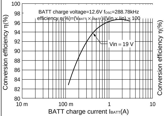
Conversion efficiency vs. charge current
