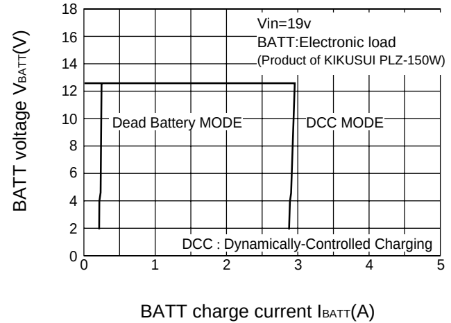
BATT voltage vs. BATT charge current
