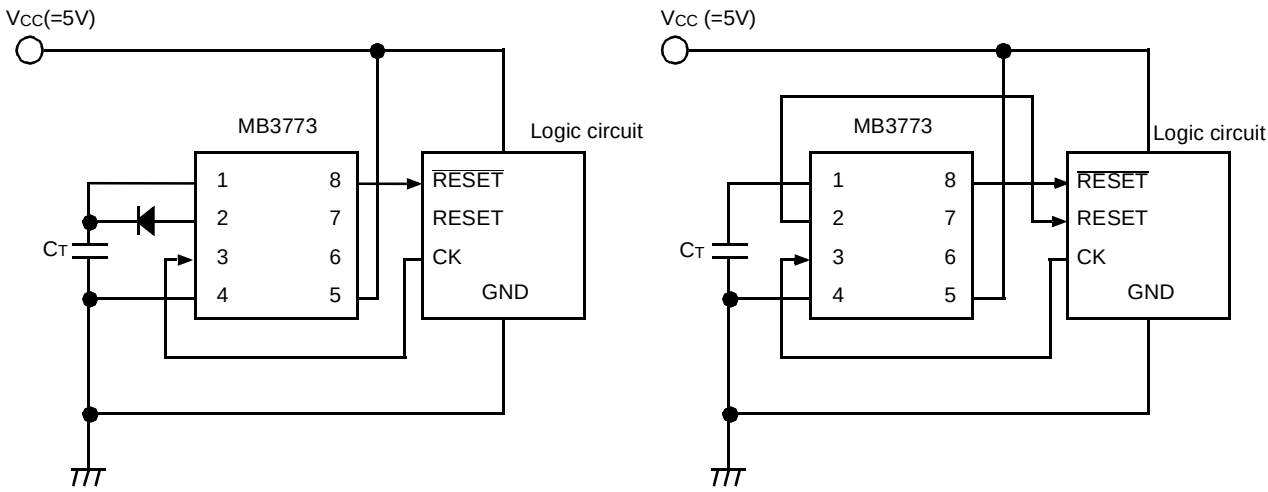
EXAMPLE 9 : Reducing Reset Hold Time
