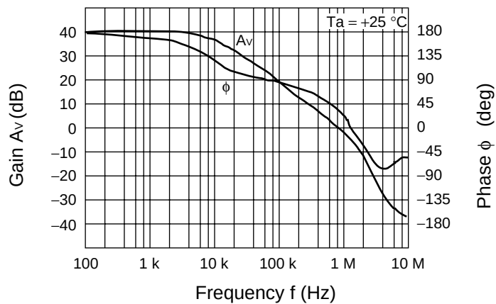
Error amplifier, gain and phase vs. frequency (ch1)
