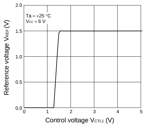
Reference voltage vs. control voltage
