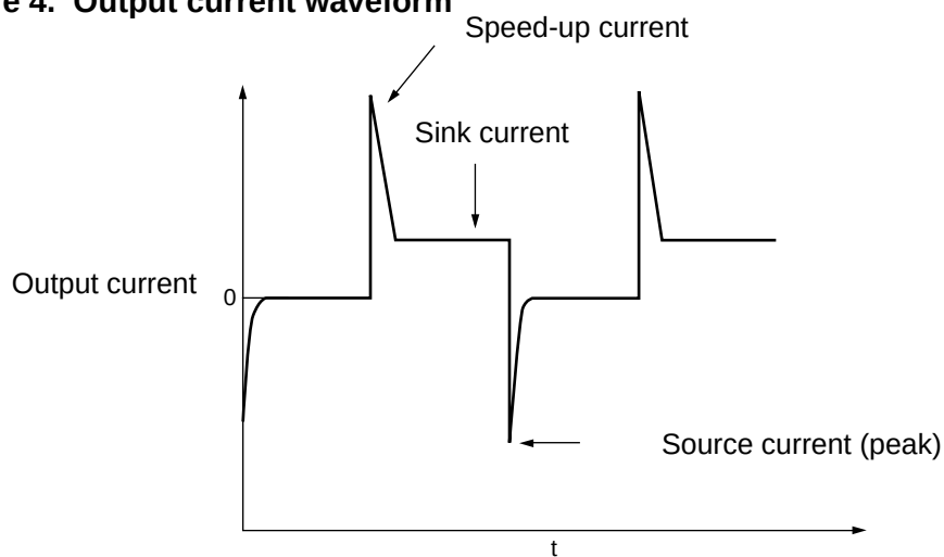
Figure 4. Output current waveform
