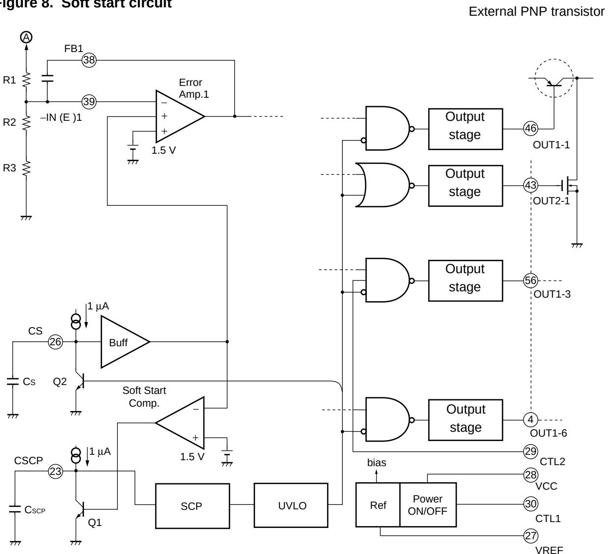
Figure 8. Soft start circuit
