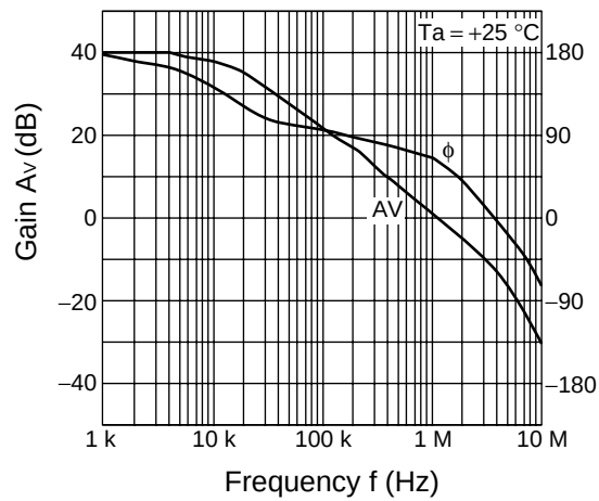
Error amplifier gain and phase vs. frequency (ch5)
