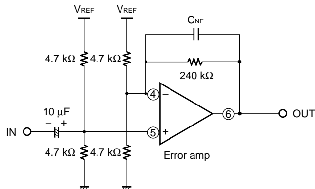
Test Circuit
