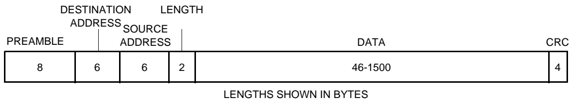
Figure 7 Packet Format
