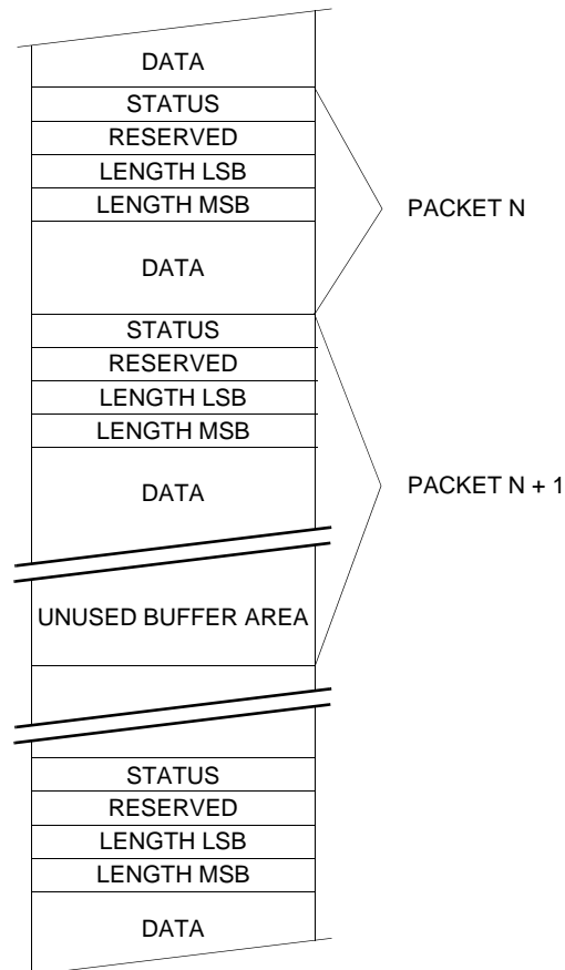
Figure 6 Receive Buffer Detail
