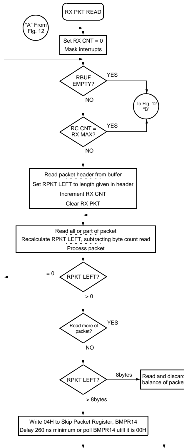
Figure 14 Receive Packet Read Routine
