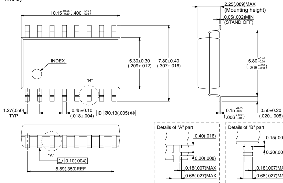
16-pin Plastic SOP (FPT-16P-M06)
