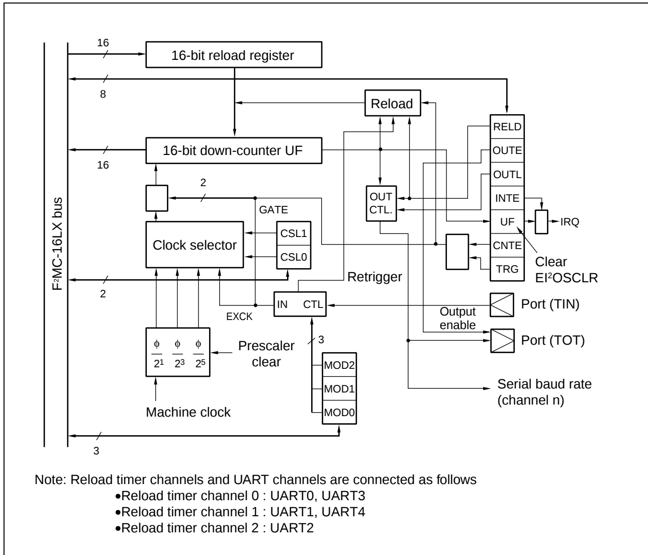
(2) Block Diagram
