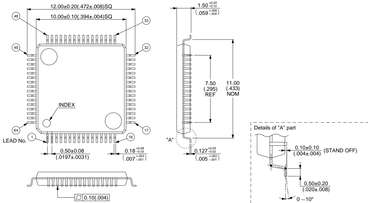
64-pin Plastic SQFP (DIP-64P-M03)
