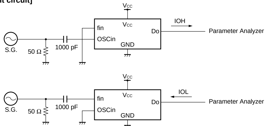
[Measurement circuit]
