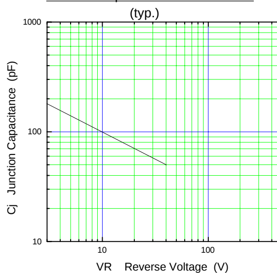
Junction Capacitance Characteristic
