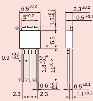
K-pack(L): Power MOSFET K-pack(P): Diode
