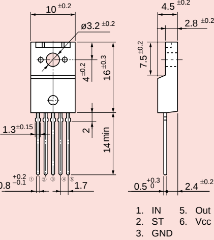
TO-220F5
