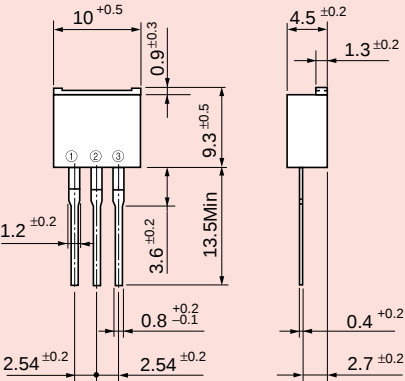
T-pack(L): Power MOSFET Transistor, IGBT T-pack(P): Diode
