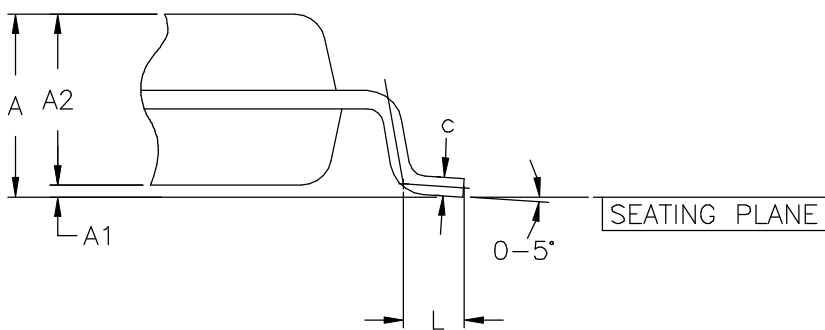
DETAIL A
