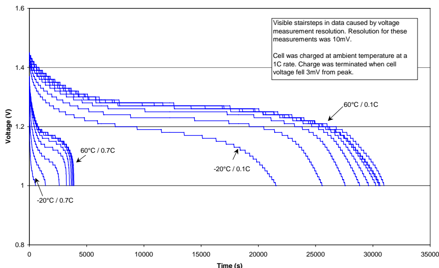
Figure 1: NiMH Discharge over Temperature (0.1C/0.7C)
