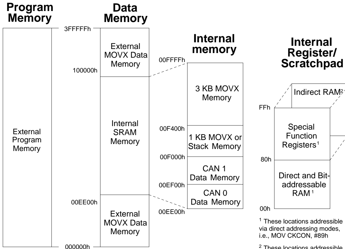
Figure 4- 1 DS80C390 Memory Map (Default Settings)
