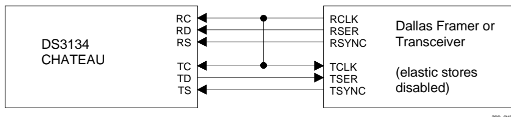
Single T1/E1 Line Connection
