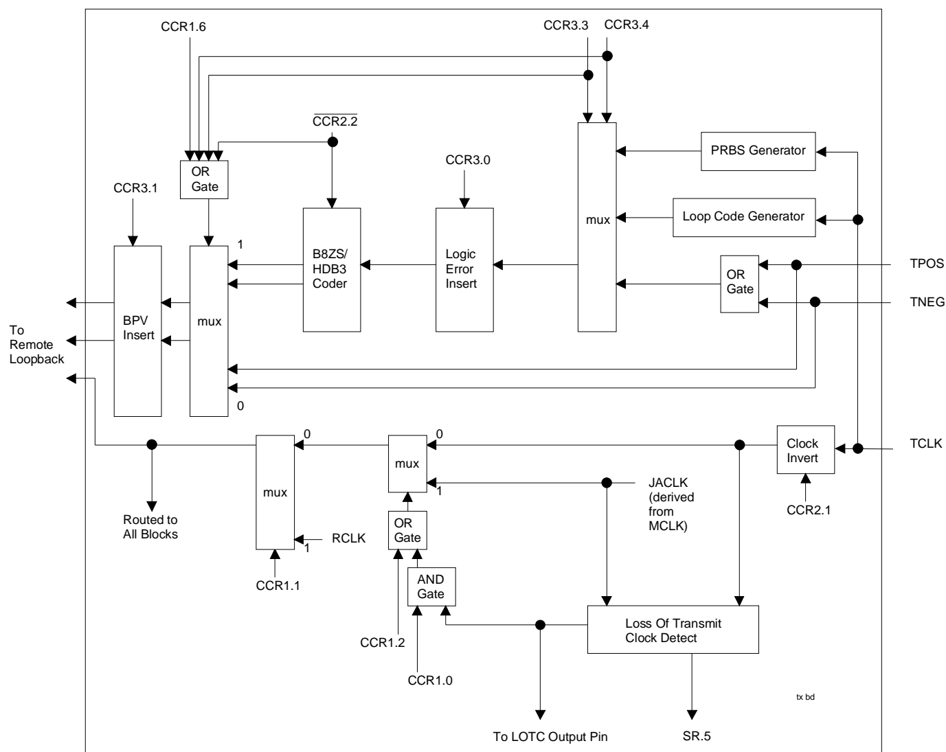
Figure 3-3 TRANSMIT LOGIC
