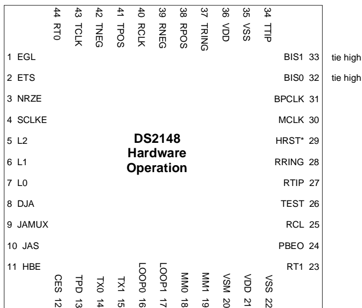
Figure 4-3 HARDWARE MODE PINOUT (BIS1 = 1, BIS0 = 1)
