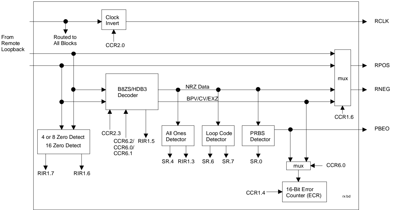
Figure 3-2 RECEIVE LOGIC
