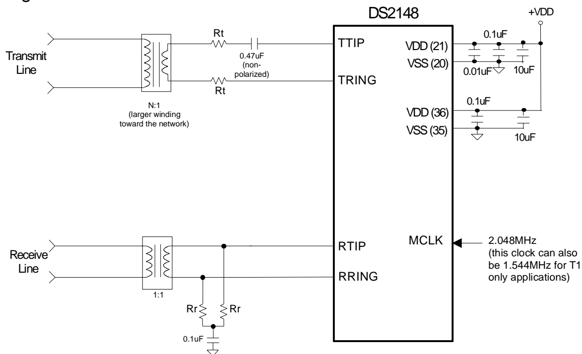
Figure 9-1 BASIC INTERFACE
