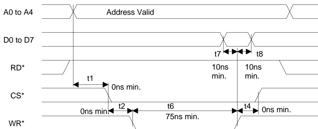
Figure 12-5 INTEL BUS WRITE TIMING (PBTS = 0, BIS1 = 0, BIS0 = 1)
