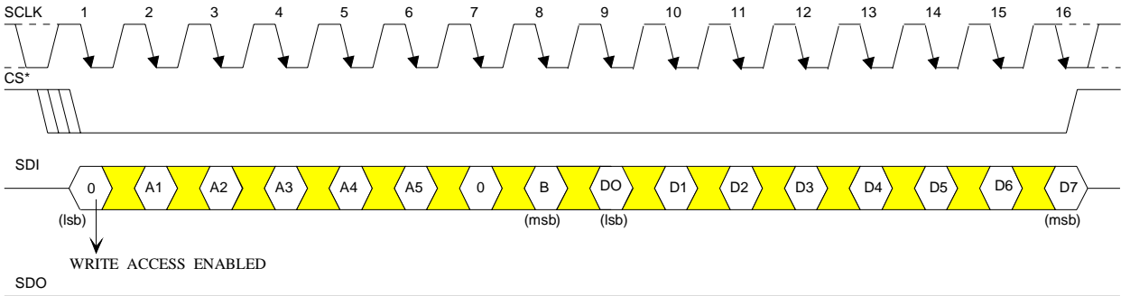
Figure 5-5 SERIAL PORT OPERATION FOR WRITE ACCESS (R=0) MODES 1 & 2
