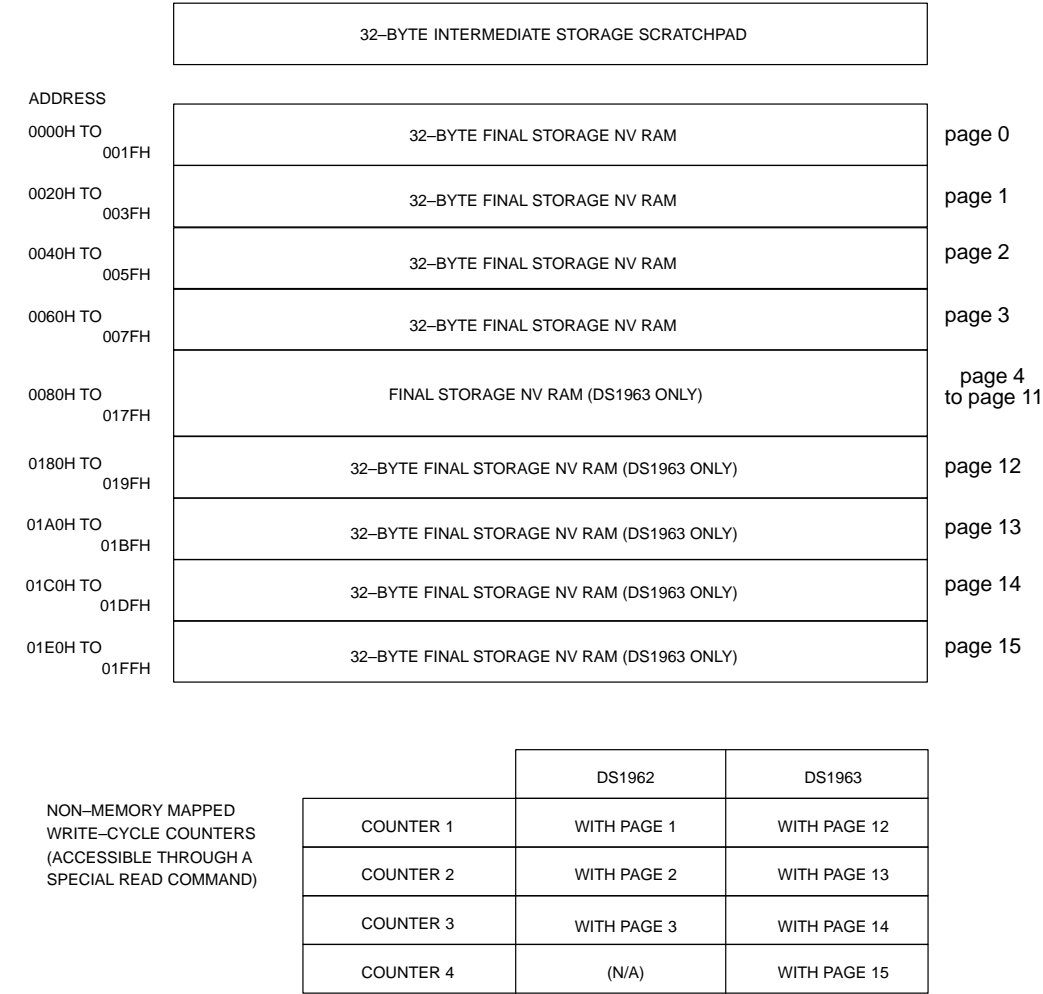
DS196X MEMORY MAP Figure 5
