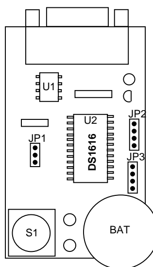
Figure 2. DS1616 Evaluation Board
