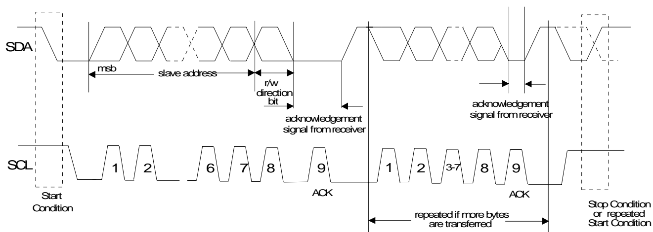
Figure 3 COMMAND/CONTROL BYTE
