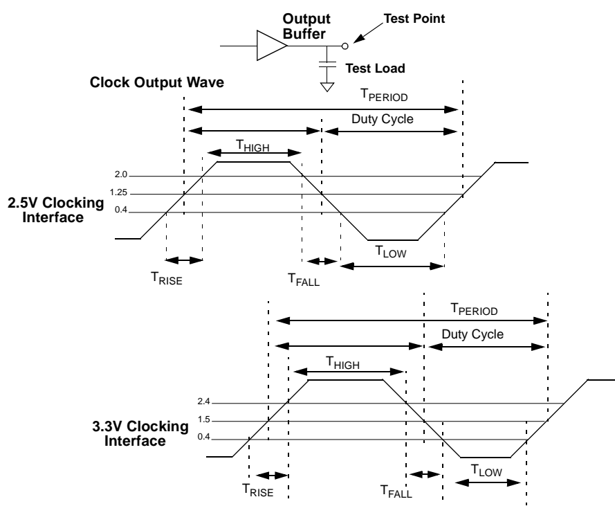
Figure 10. Output Buffer
