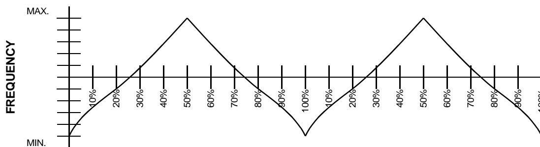
Figure 7. Typical Modulation Profile
