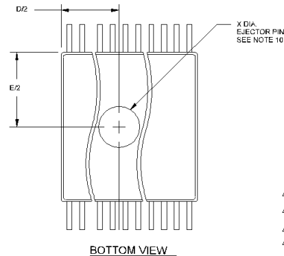
48-Pin Shrink Small Outline Package (SSOP, 300 mils)
