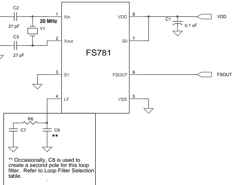
Figure 5. FS781 Schematic
