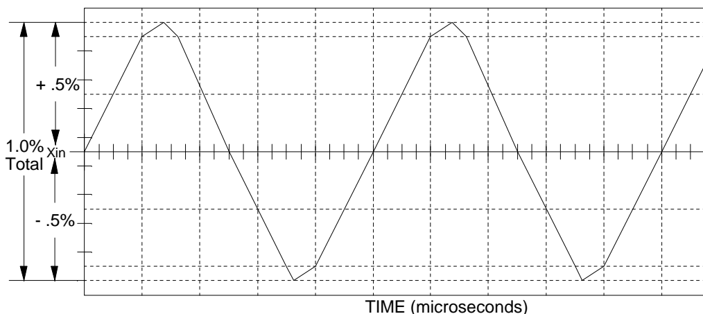
Figure 1. Frequency Profile in Time Domain [9]
