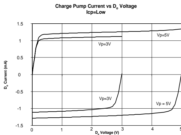
Figure 3. D_o Output Current Low Mode
