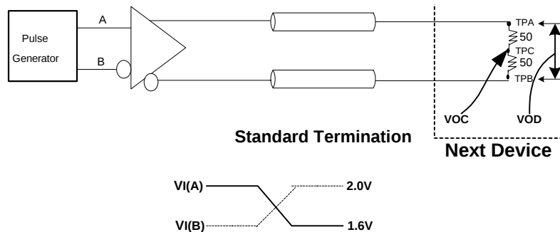
Figure 2. Test Circuit and Voltage Definitions for the Driver Common-mode Output Voltage [2,3,4,5]
