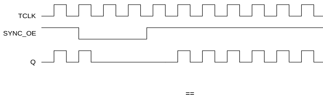
Figure 1. SYNC_OE Timing Diagram
