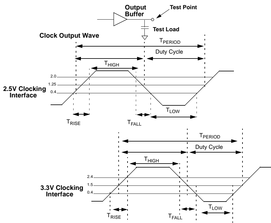
Figure 1. Output Buffer
