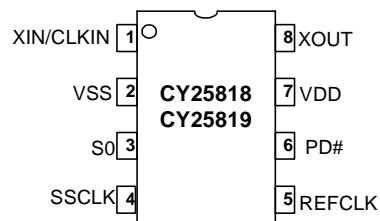
8-pin SOIC
