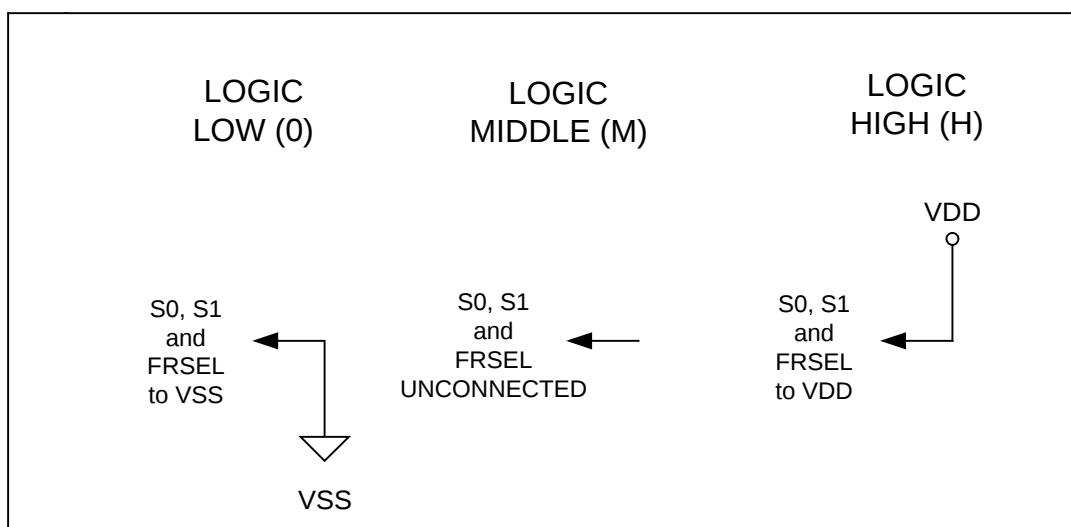
Figure 3. 3-Level Logic
