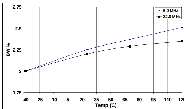
Figure 4B. Bandwidth % vs. Temperature
