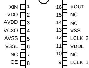
CY2413-2 16-pin TSSOP
