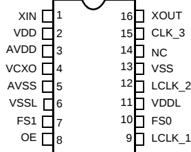
CY2413-1 16-pin TSSOP
