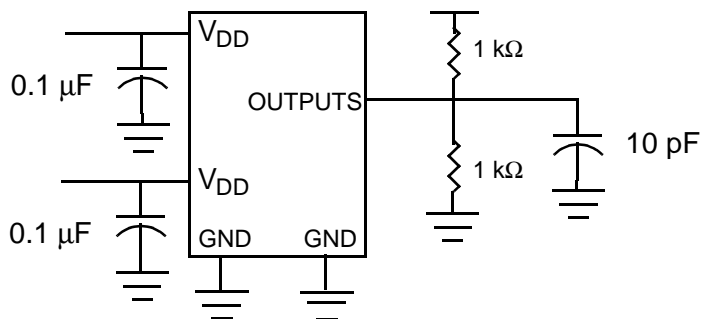
Test Circuit # 2
