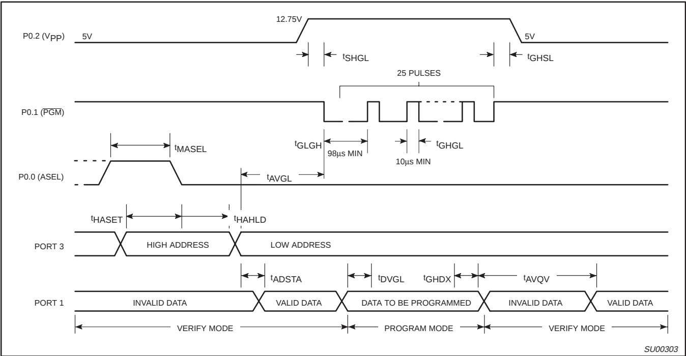
Figure 7. Program/Verify Cycle
